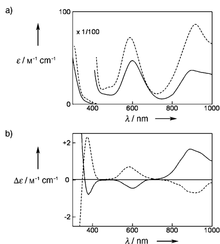
Figure 2. a) Absorption and b) CD spectra of 1^{5-} ( (\Lambda)_2[\text{Au}_3\{\text{Ni}(\text{L-cys})_3\}_2]^{5-} , —) and 2^{5-} ( (\Delta)_2[\text{Au}_3\{\text{Ni}(\text{L-pen})_3\}_2]^{5-} , ----) in water.
