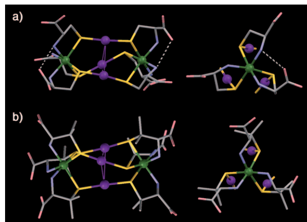
Figure 3. Perspective views of a) 1^{5-} and its [\text{Au}_3\{\text{Ni}(\text{L-cys})_3\}] moiety, and b) 2^{5-} and its [\text{Au}_3\{\text{Ni}(\text{L-pen})_3\}] moiety. Au purple, Ni green, S yellow, O red, N blue, C gray. Hydrogen atoms are omitted for clarity. Dotted line represents the intramolecular hydrogen bonds between carboxylate and amine groups.
